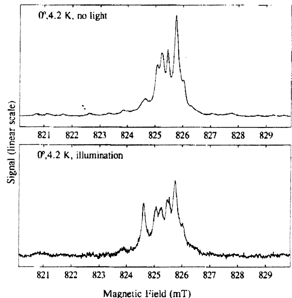
Fig. 5. Influence of white light illumination on spectrum II as measured at 23 GHz microwave frequency and 4.2 K.
