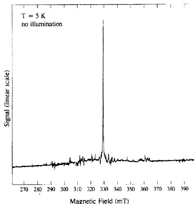
Fig. 8. EPR spectrum of heat-treated sample as measured at 9.2 GHz microwave frequency and liquid helium temperature.
