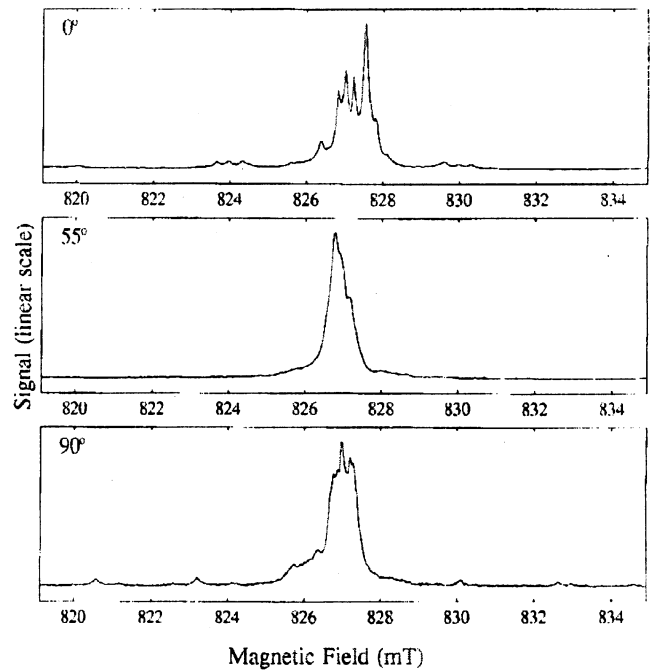
Fig. 4. Spectrum II as recorded at 23 GHz microwave frequency in three different directions of the magnetic field.
