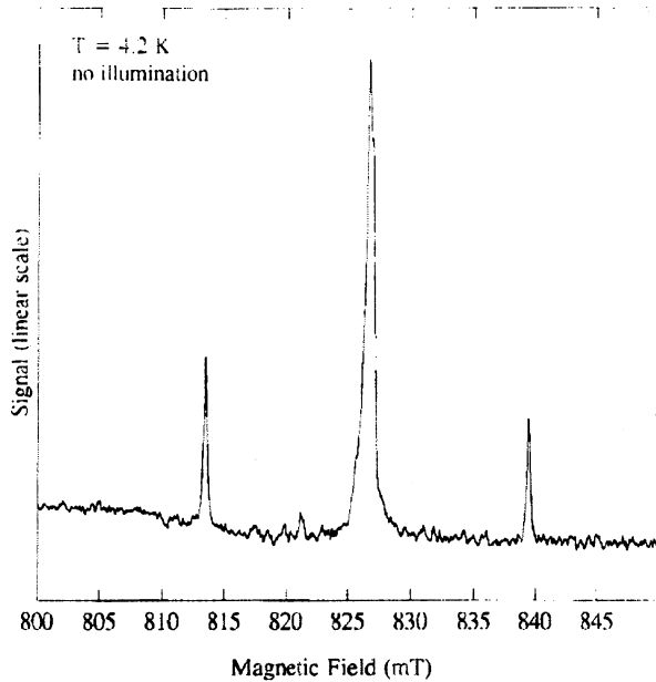
Fig. 2. EPR spectrum of heat-treated sample as measured at 23 GHz microwave frequency (without illumination) at 4.2 K.
