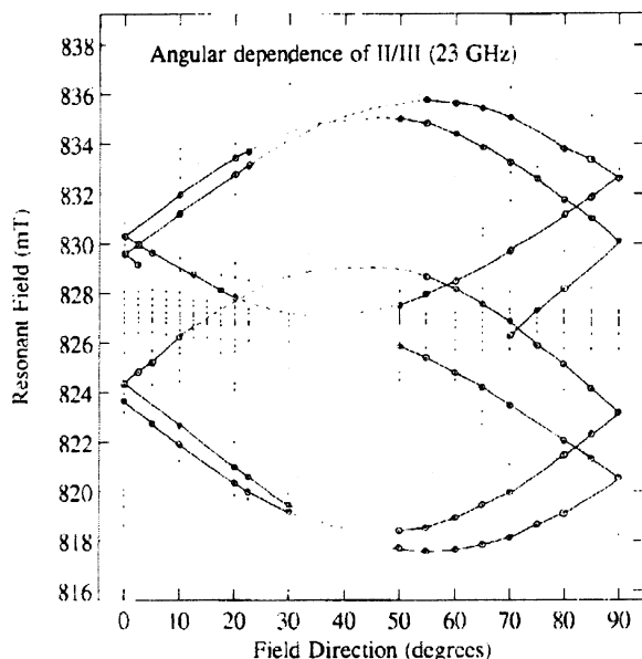
Fig. 7. Angular dependence of spectrum II as measured at 23 GHz microwave frequency (without illumination) and 4.2 K. The magnetic field has been rotated in the plane as indicated on Fig. 1.
