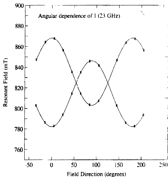
Fig. 3. Angular dependence of spectrum I as measured at 23 GHz microwave frequency and 4.2 K. The magnetic field has been rotated in the plane as indicated on Fig. 1.
