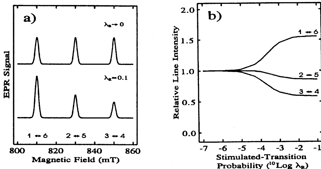
Figure 5 a) Low power spectrum (top trace) and saturated spectrum (bottom trace). The nuclear spin is polarized by the microwaves. b) Microwave-power dependence of the individual line intensities.
