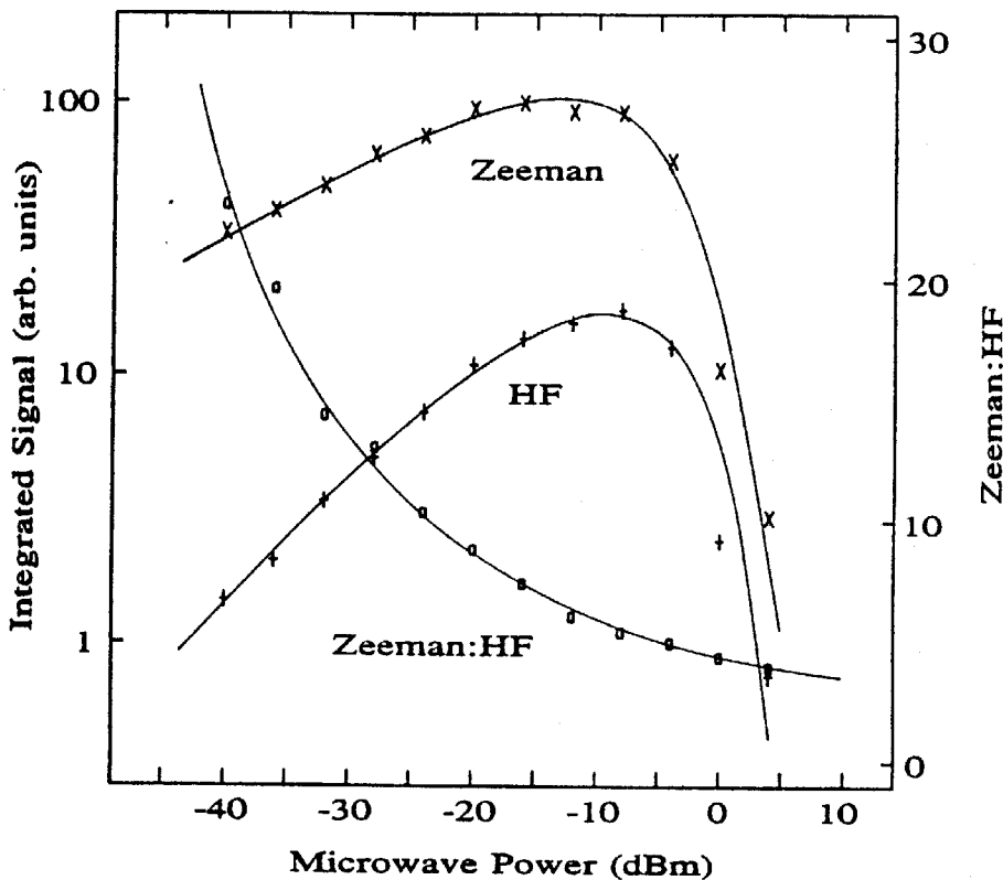
Figure 3 Microwave power dependence of the Zeeman and HF components of Si-NL52. The ratio is changing even before saturation sets in.
