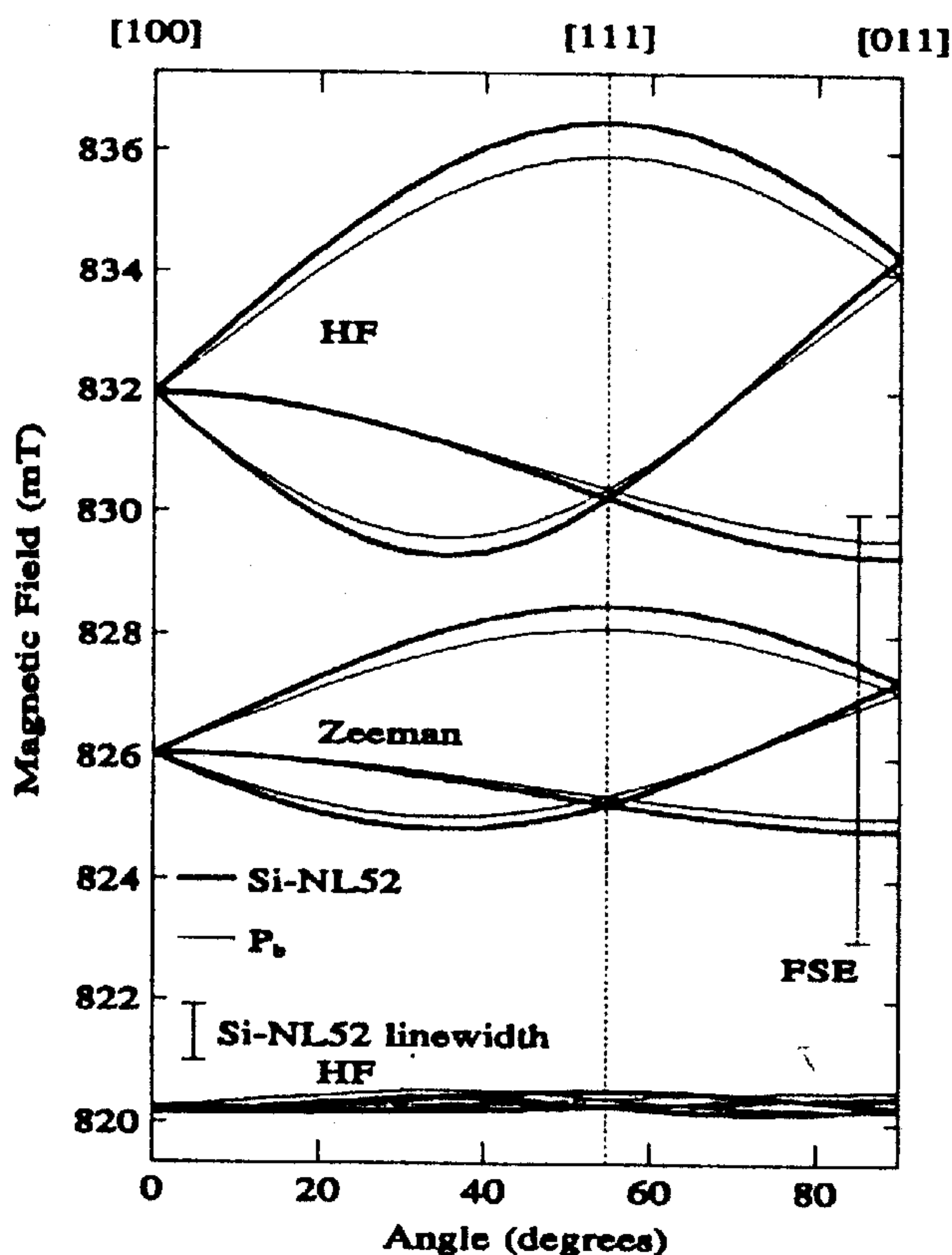
Figure 2 Simulations of the Si-NL52 (thick trace) and P_b spectra (thin trace) for a microwave frequency of 23.2 GHz. The place of the FSE scan of Figure 6 is indicated with a dashed line.
