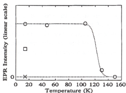
Fig. 2. Thermal quenching of the photo-induced EPR spectrum in AlSb:Se measured at 14 K. The figure shows the EPR intensity for cooling in the dark ( \times ), during illumination ( \square ), and after switching off the light ( \circ ). To return the sample to the nonparamagnetic state it has to be heated to a temperature above 115–130 K.
